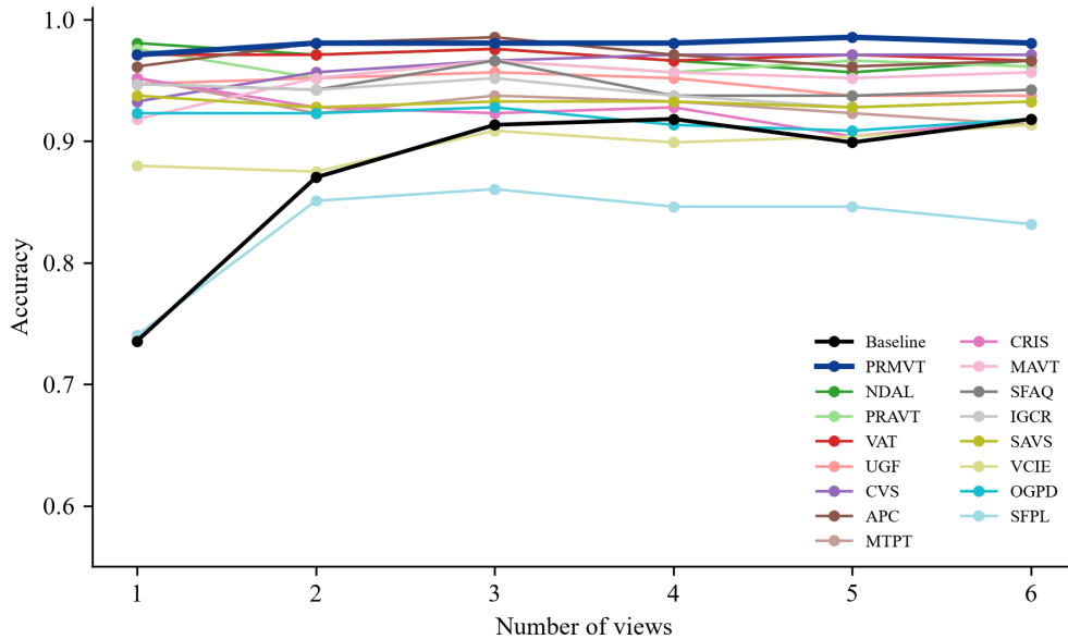
Figure 18: Authentication accuracy against the number of views for the CNN+ViT baseline, PRMVT and the other training variants tried in this project
