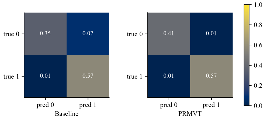
Figure 19: Normalised confusion matrices of the baseline and PRMVT at six views (0 = counterfeit, 1 = genuine)
