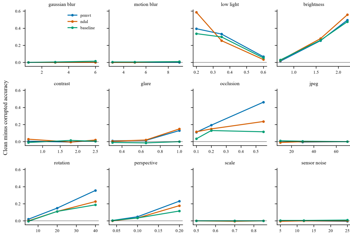
Figure 20: Accuracy drop (clean minus corrupted accuracy) at six views under 12 corruptions for PRMVT, the NDAL variant and the baseline
