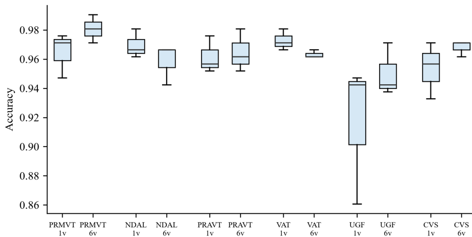
Figure 24: Spread of test accuracy over seeds 42, 43 and 44 at one view (1v) and six views (6v) for the main training variants
