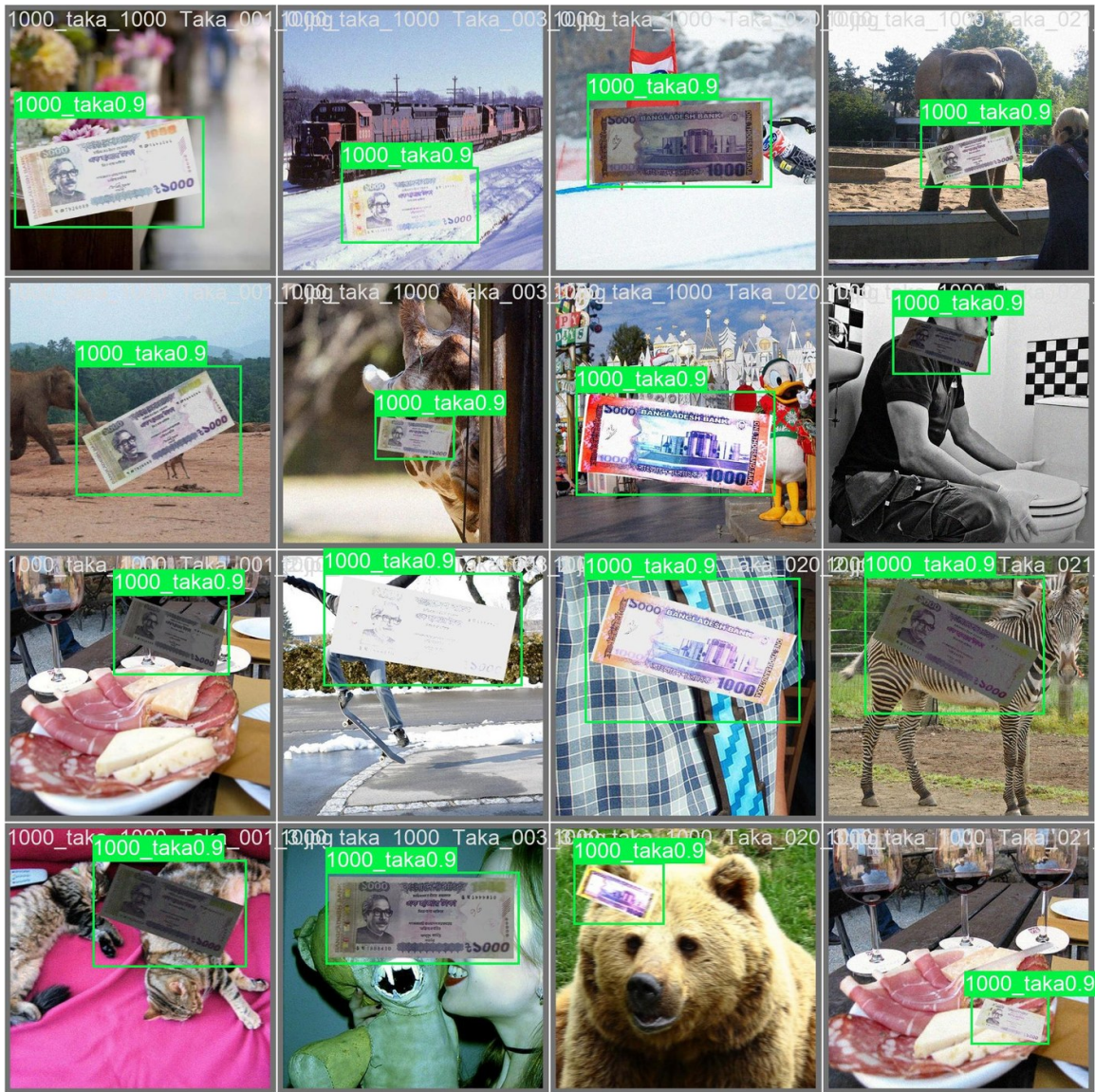
Figure 16: Example predictions on held-out composites with predicted class and confidence. The note is localised across different scales, rotations and backgrounds.
