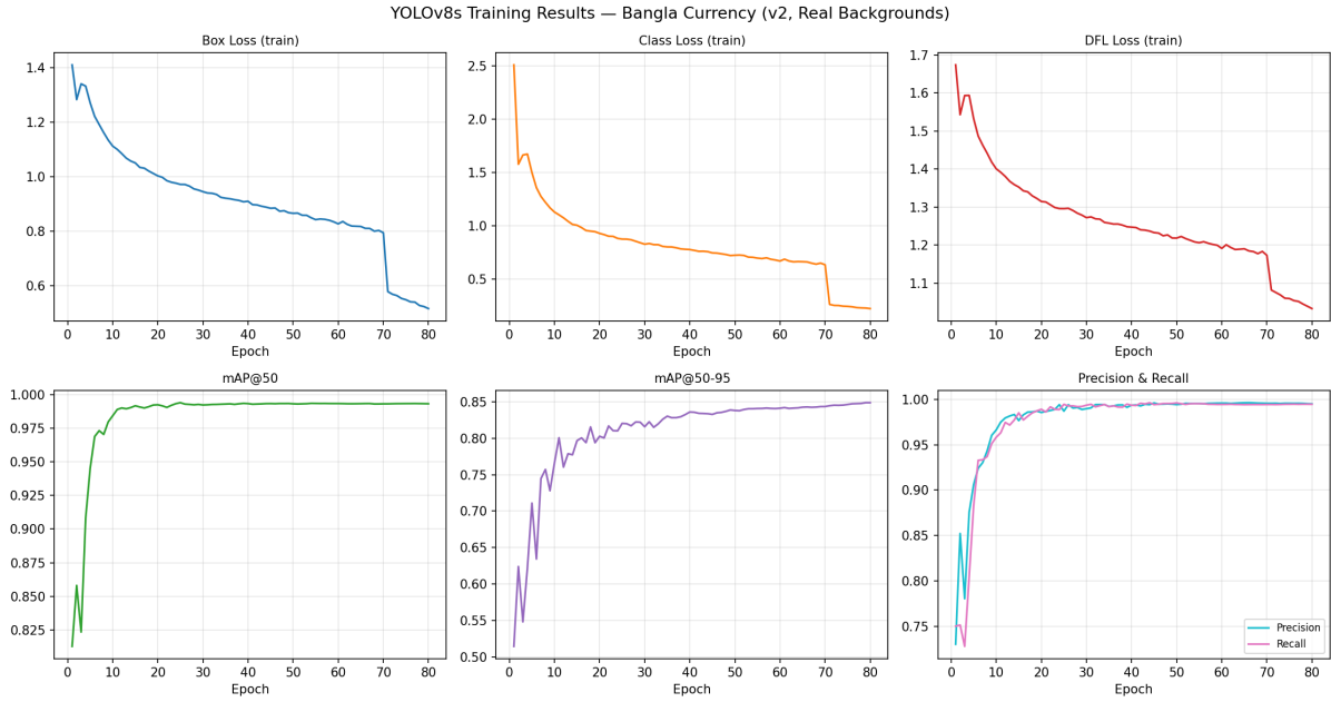
Figure 14: Training curves of the YOLOv8s Taka detector: box, class and DFL losses (top) and mAP@0.5, mAP@0.5:0.95, precision and recall (bottom) against epoch
