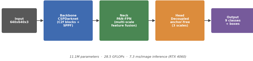
Figure 4: YOLOv8s detection architecture used for Taka detection: CSPDarknet backbone, PAN-FPN neck and decoupled anchor-free head predicting 9 classes and box coordinates
