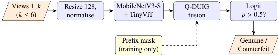
Figure 5: Multi-view currency authenticator. During prefix-robust training, a random prefix of 1 to 6 views is kept so the model learns to decide with any number of views.
