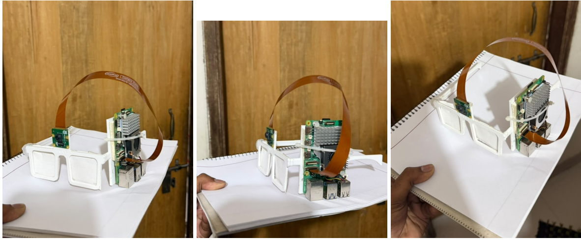
Figure 3: First prototype of Savior Glass: the camera module above the bridge of a 3D-printed frame (left), the Raspberry Pi 5 with heat sink and fan tied to the right temple (centre), and the ribbon cable between camera and board (right)
