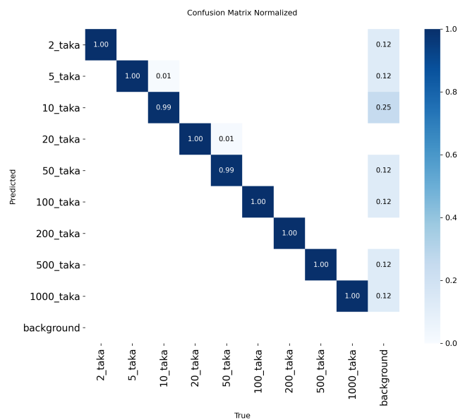
Figure 15: Normalised confusion matrix of the Taka detector on the synthetic test set
