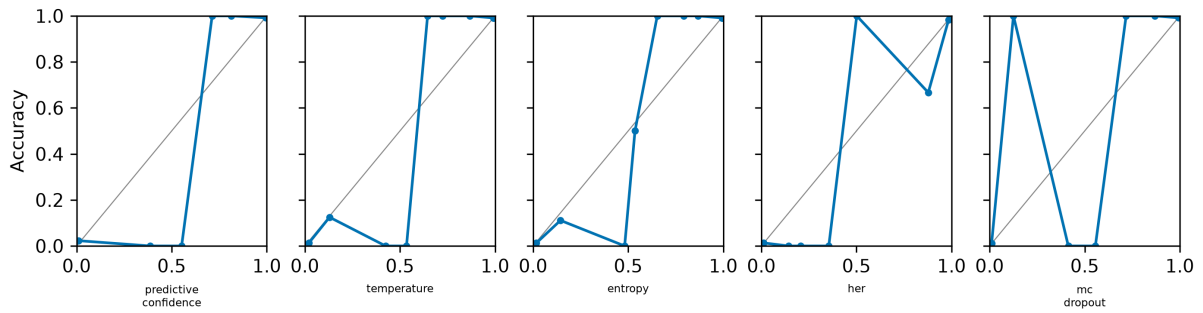
Figure 23: Reliability diagrams of the authenticator at six views for five confidence estimates (raw predictive confidence, temperature scaling, entropy mapping, HER and MC dropout); calibration maps fitted on the validation split and evaluated on the test split
